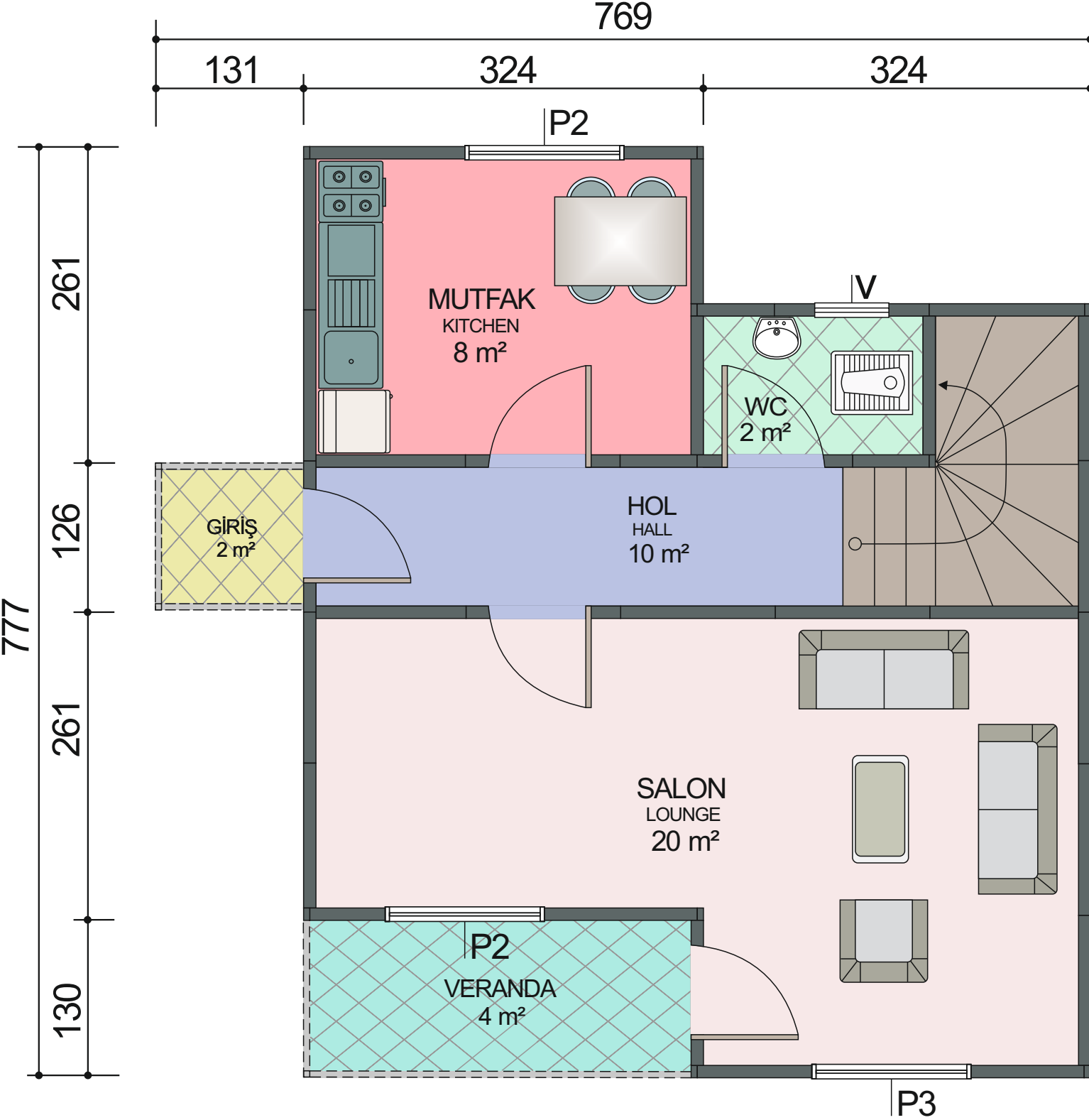
ZEMİN KAT PLANI GROUND FLOOR PLAN 41 \text{ m}^2 + 6 \text{ m}^2 = 47 \text{ m}^2
